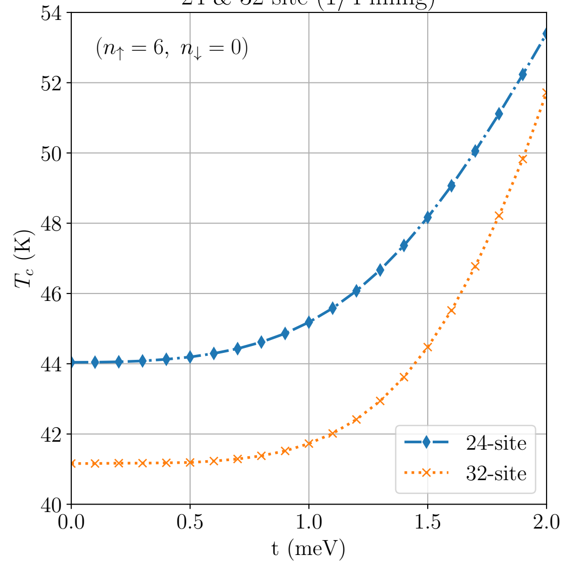
24 &amp; 32-site (1/4 filling)
