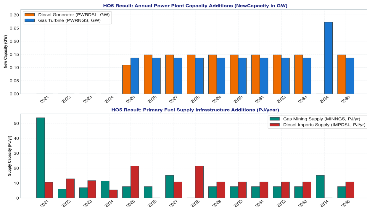
Figure: Top: Annual power plant additions (GW). Bottom: Primary gas mining and diesel import supply infrastructure (PJ/yr).
