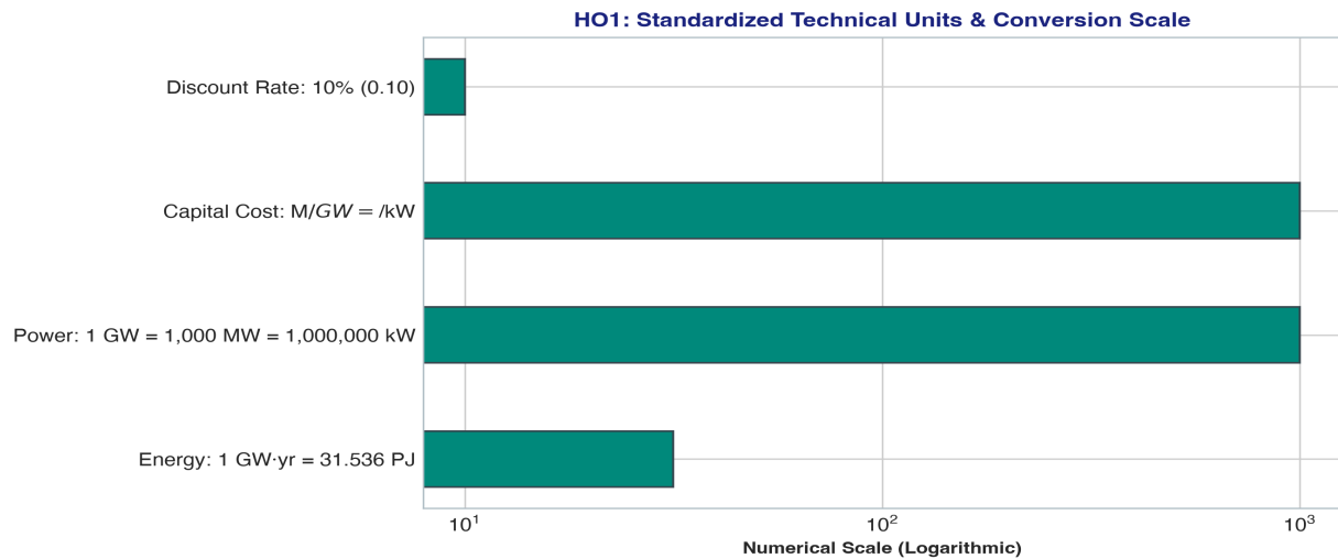
Figure: Technical units standardization framework in OSeMOSYS.
