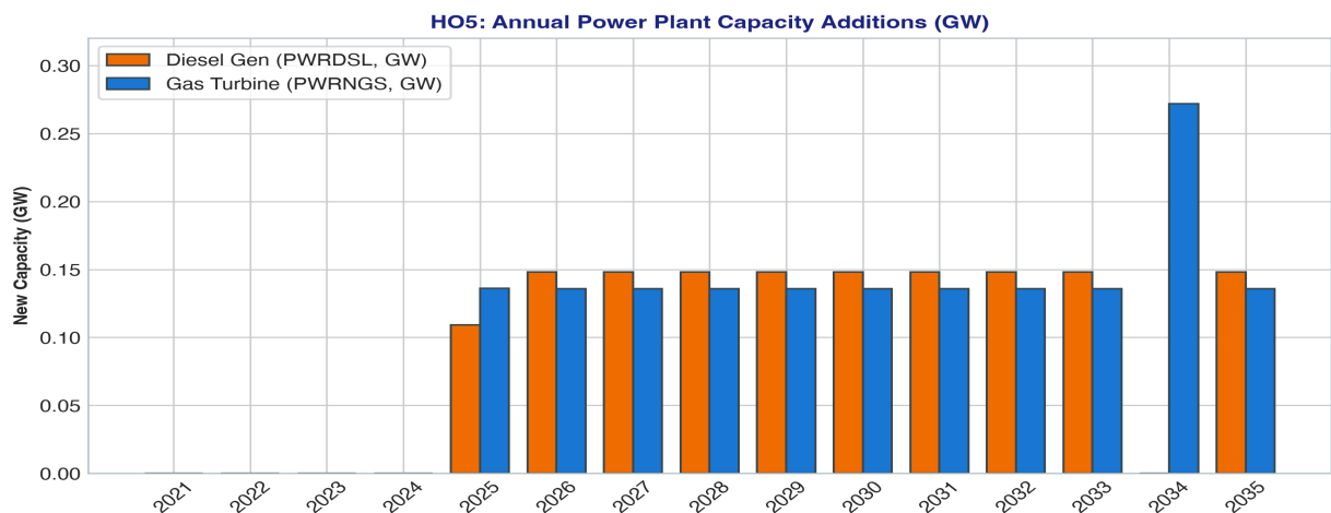
Figure: Annual capacity additions of gas turbines and diesel generators (GW).
