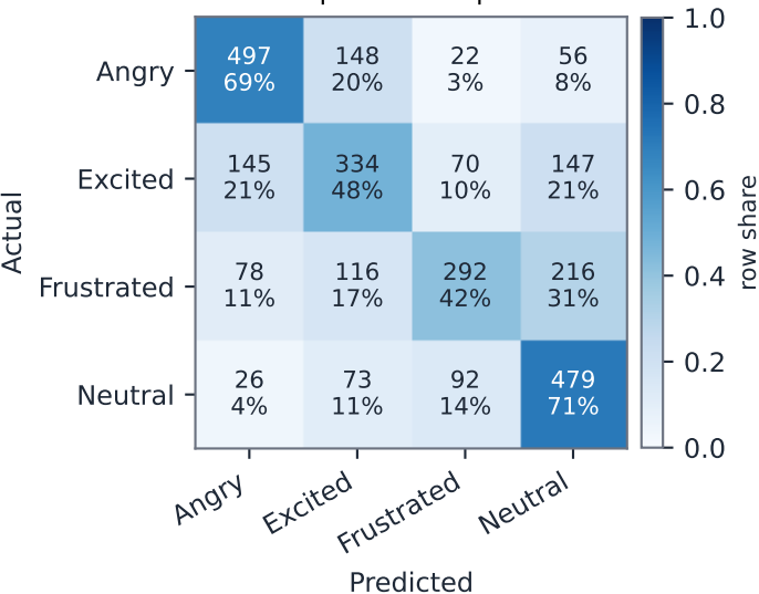
Voice model — speaker-independent confusion
