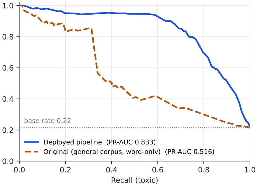
Precision (toxic)
