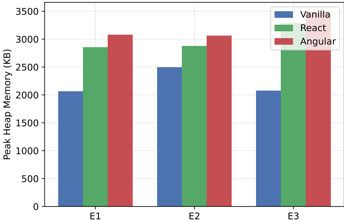
Median Peak Heap Memory by Framework and Environment
