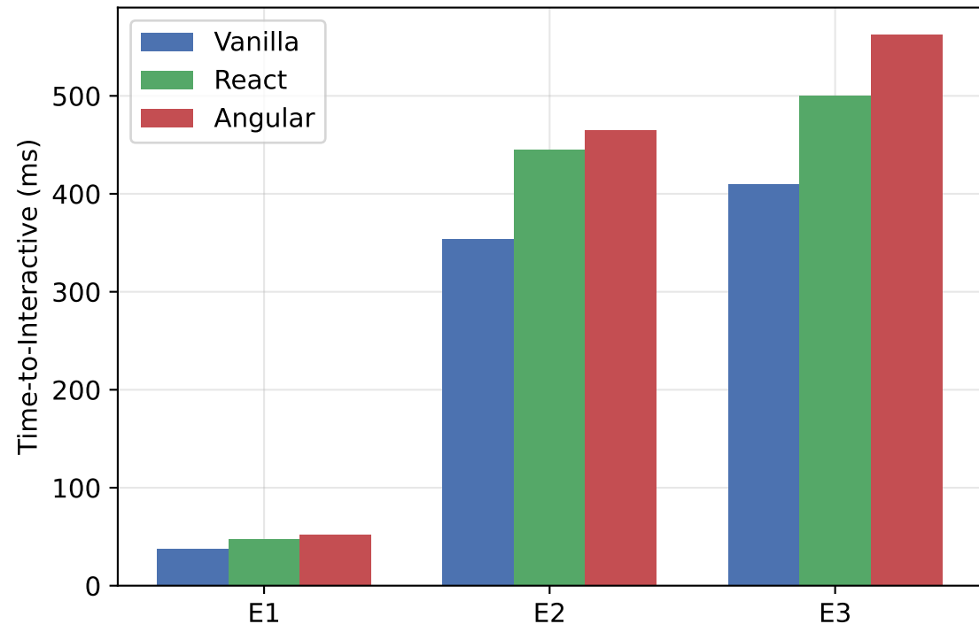
Median Time-to-Interactive by Framework and Environment
