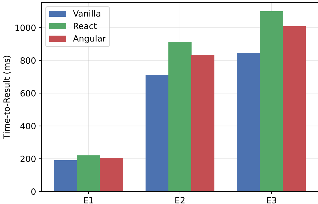
Median Time-to-Result by Framework and Environment
