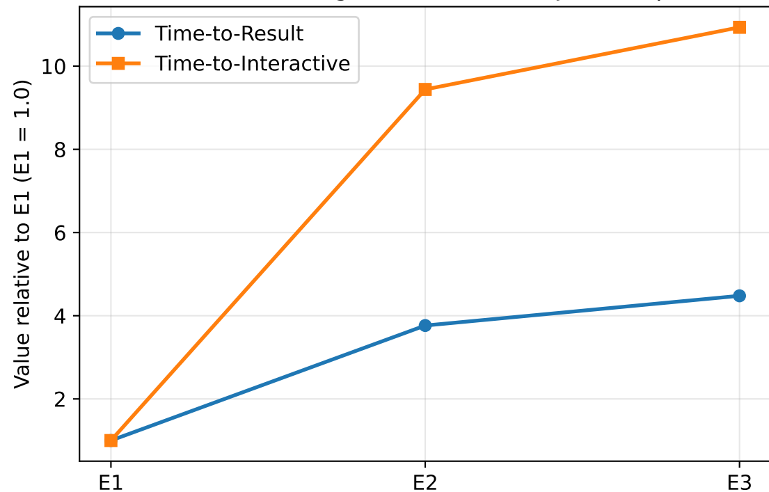
TTR vs. TTI Degradation (Vanilla JavaScript)
