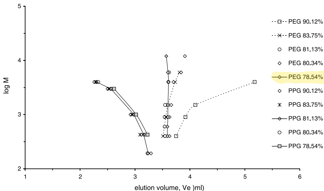
Fig. 8. Elution volumes of PEG and PPG with different molar mass on the Diol column in acetone–water mobile phases of different composition (in wt%).
