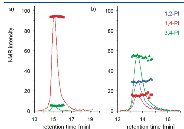
Figure 5. NMR chromatograms (normalized to 100%) at critical conditions of 1,4-PI for (a) 1,4-PI sample ( M_n = 20.7 \text{ kg mol}^{-1} ) and (b) 3,4-PI sample ( M_n = 33.0 \text{ kg mol}^{-1} ); blue solid line = NMR elution of 1,2-isoprene units, red solid line = NMR elution of 1,4-isoprene units, green solid line = NMR elution of 3,4-isoprene units, ◆ = molar content of 1,2-PI, ■ = molar content of 1,4-PI, and ▲ = molar content of 3,4-PI.
