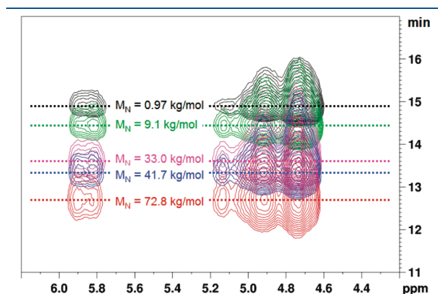
Figure 6. On-flow LCCC-NMR of 3,4-PI samples of different molar masses at critical conditions of 1,4-PI.
