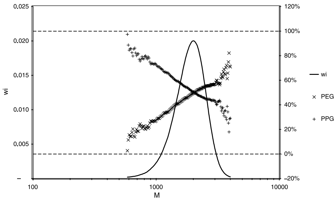
Fig. 13. MMD and chemical composition of EO–PO–EO 1900 (with 50% EO), as obtained by SEC with coupled density and RI detection (PL gel 10^3 + 10^4 Å, \text{CHCl}_3 ).
