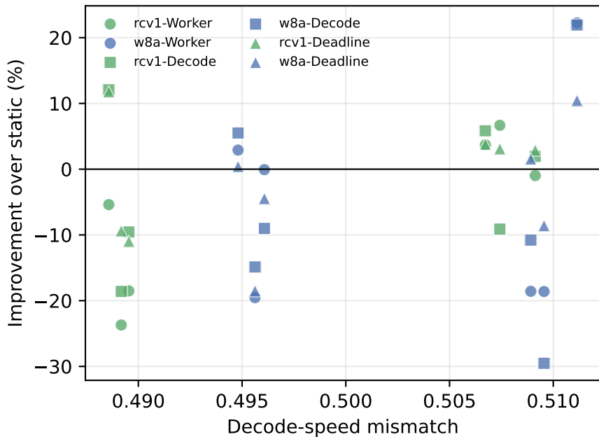
P95 improvement vs. mismatch ( r=+0.27 )
