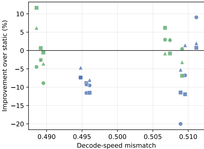
Mean improvement vs. mismatch ( r=+0.04 )
