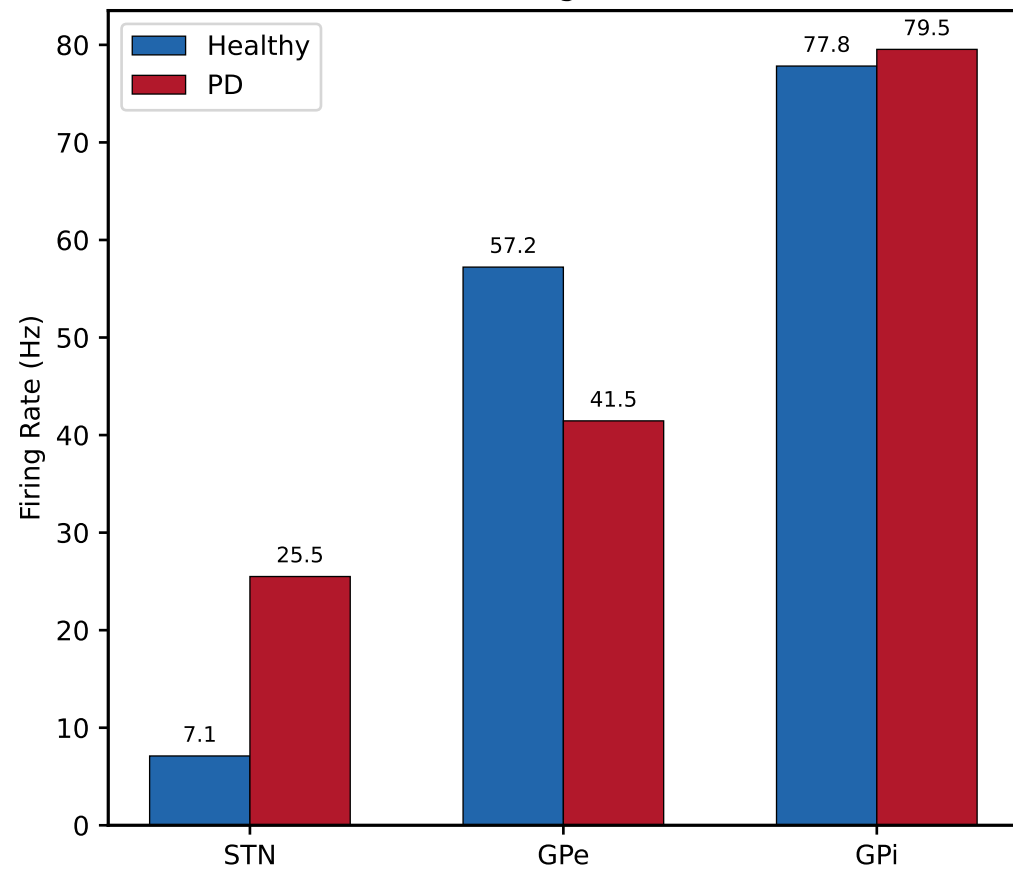
A. Firing Rates
