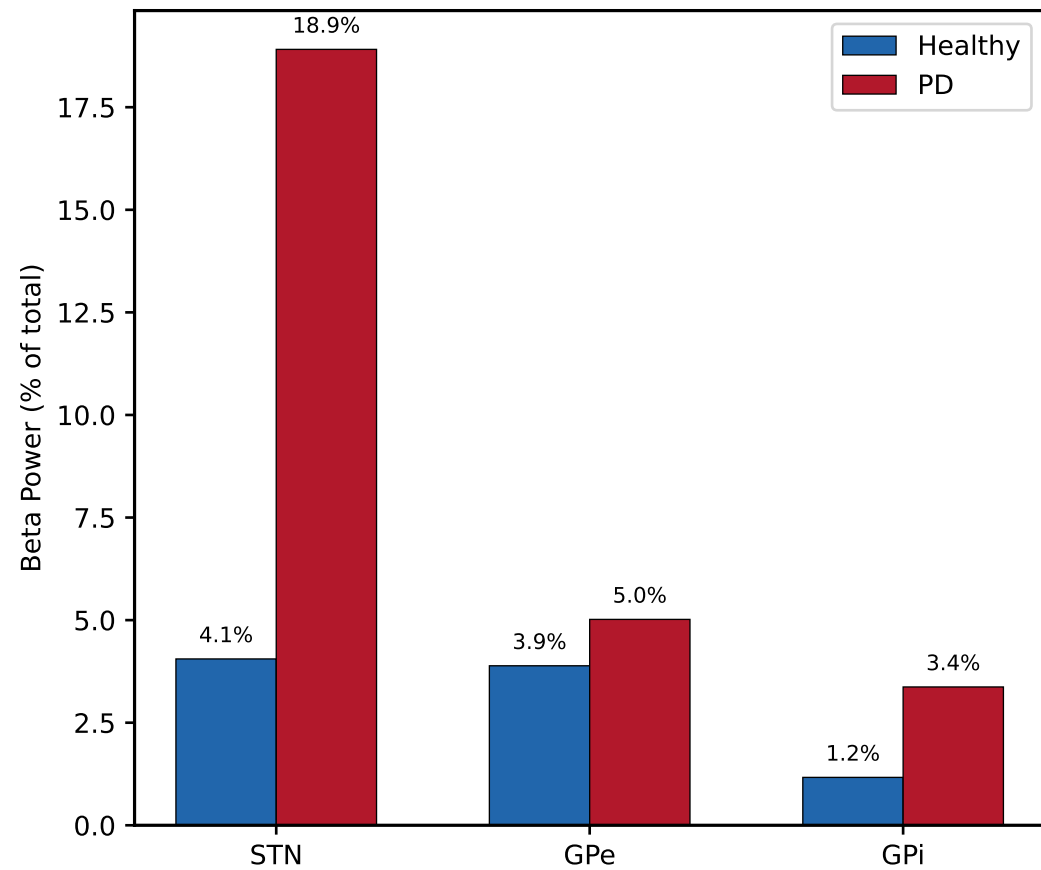
B. Beta Band Power (13-30 Hz)
