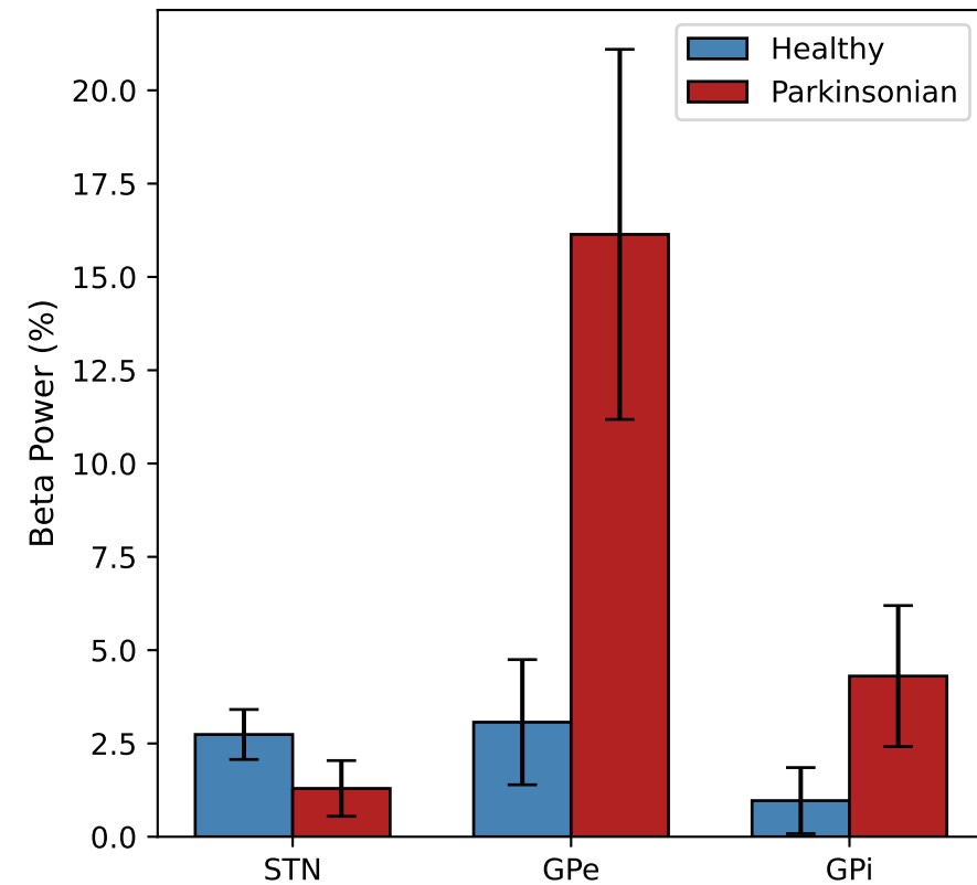
C. Beta Band Power (13-30 Hz)
