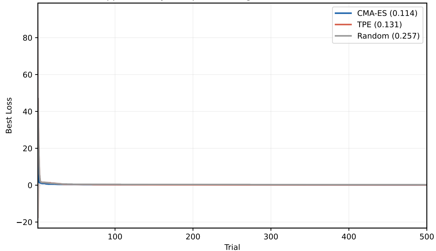
Supplementary: Sampler Convergence (5 seeds, 500 trials)
