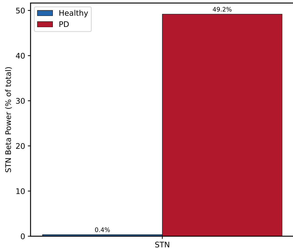
B. STN Beta Band Power (13-30 Hz)
