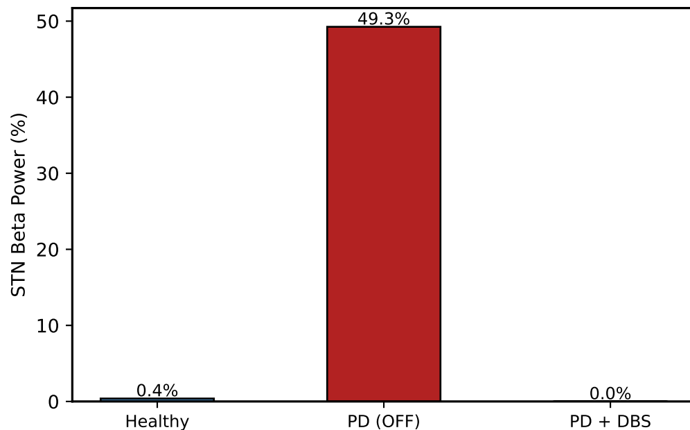
B. STN Beta Band Power
