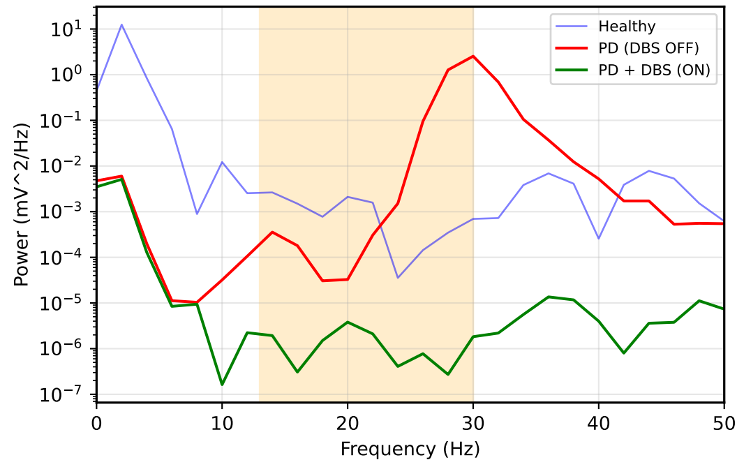
STN power spectrum Beta: 49.3% -> 0.0%
