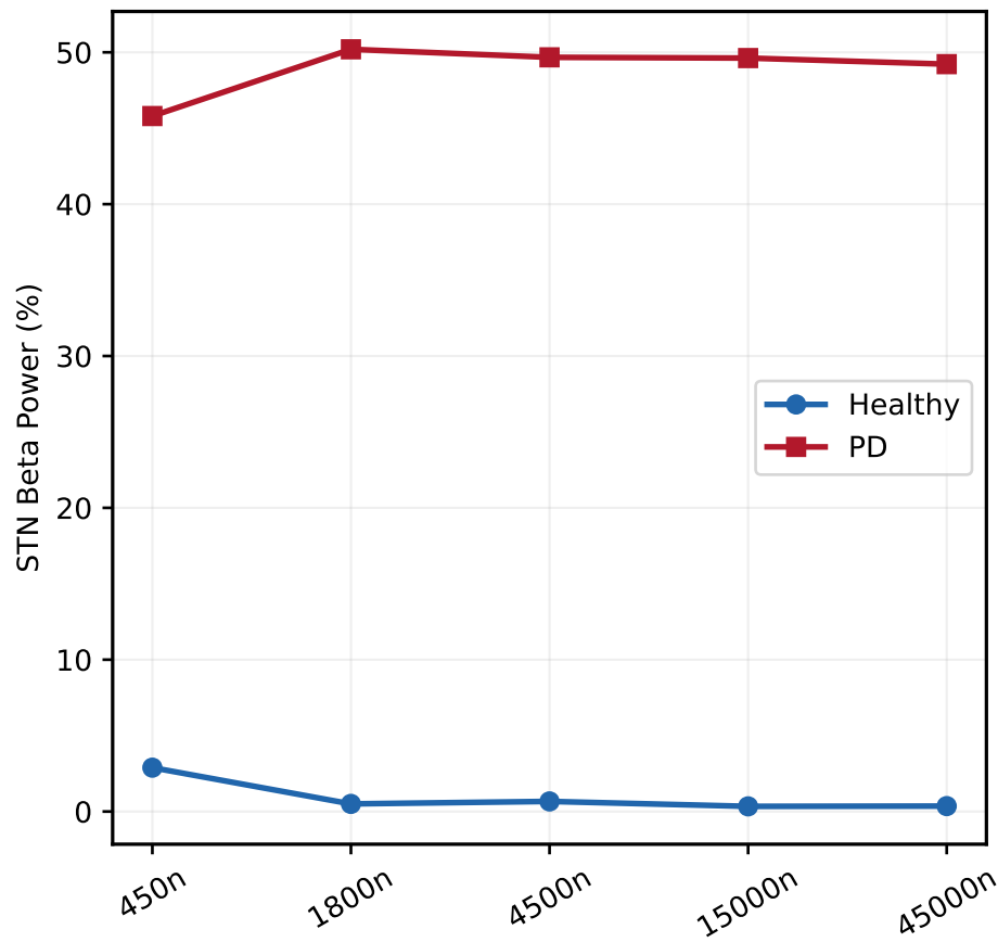
B. STN Beta vs Network Size
