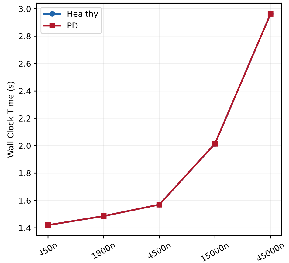
C. Simulation Time vs Network Size
