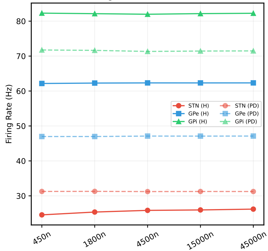
A. Firing Rates vs Network Size
