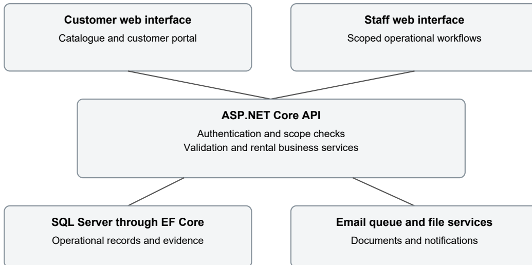
Figure 1 Logical architecture of the development system
