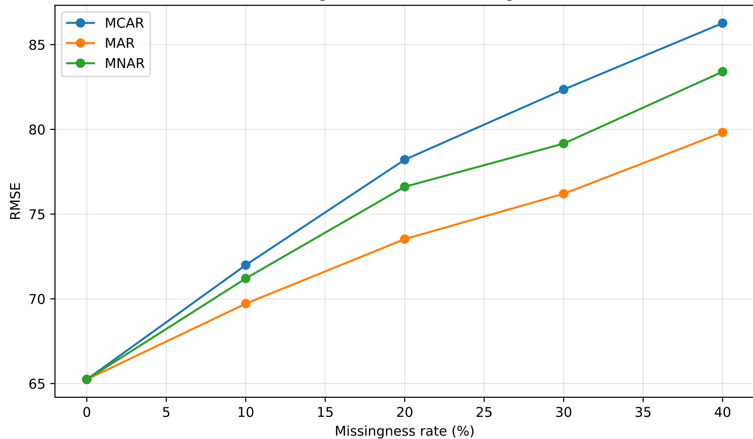
RQ1: Performance degradation under missing data mechanisms
