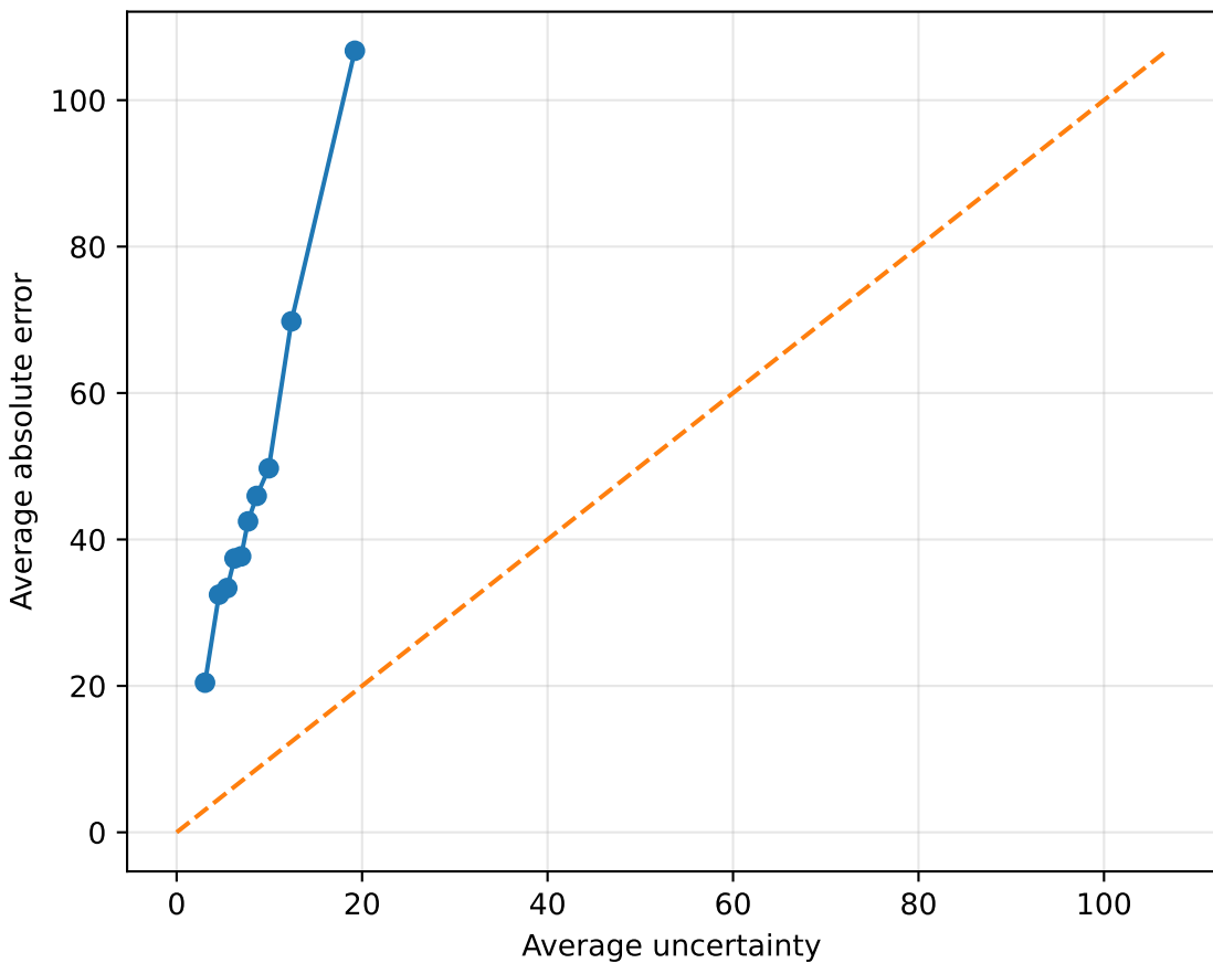
RQ3: Calibration curve
