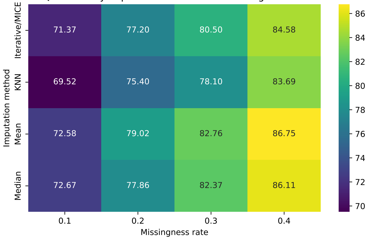
RQ4: RMSE by imputation method and missingness level
