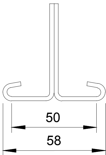
Base holder for Basket Trays
