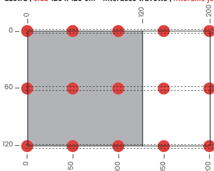
Lastra | Slab 120 x 120 cm - Interasse travetto | Interaxle joist 60 cm
