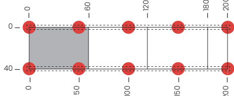
Lastra | Slab 40 x 60 cm - Interasse travetto | Interaxle joist 40 cm
