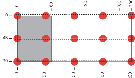
Lastra | Slab 60 x 90 cm - Interasse travetto | Interaxle joist 45 cm
