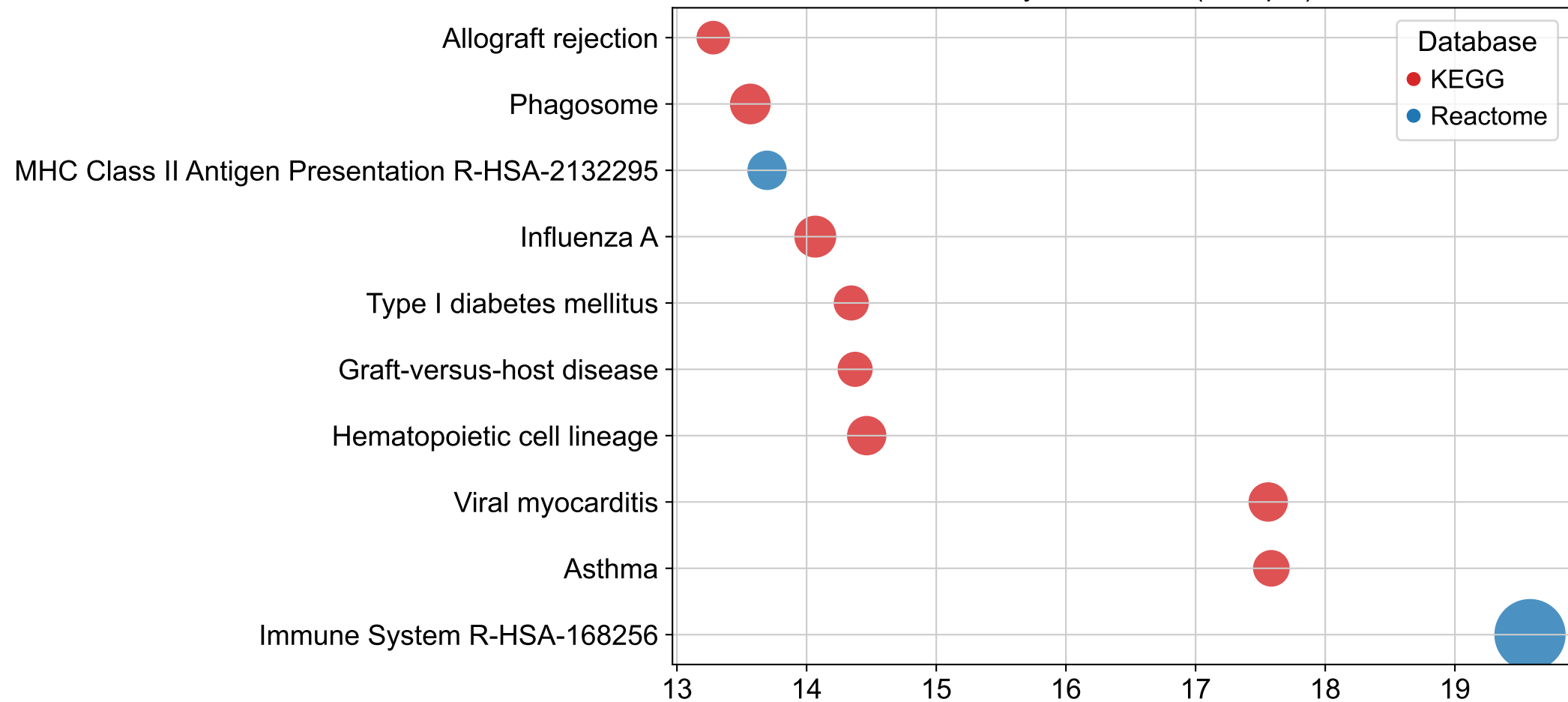
Pathway Enrichment (Group 6)
