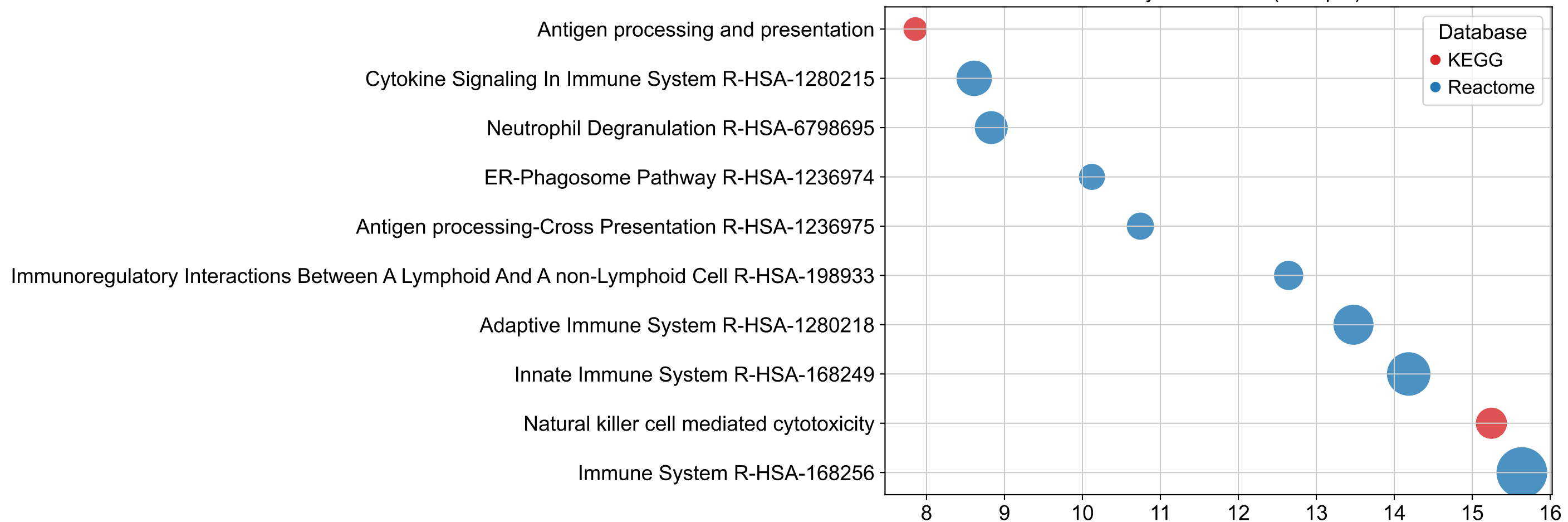
Pathway Enrichment (Group 4)
