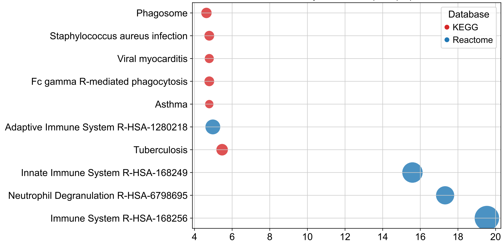
Pathway Enrichment (Group 5)
