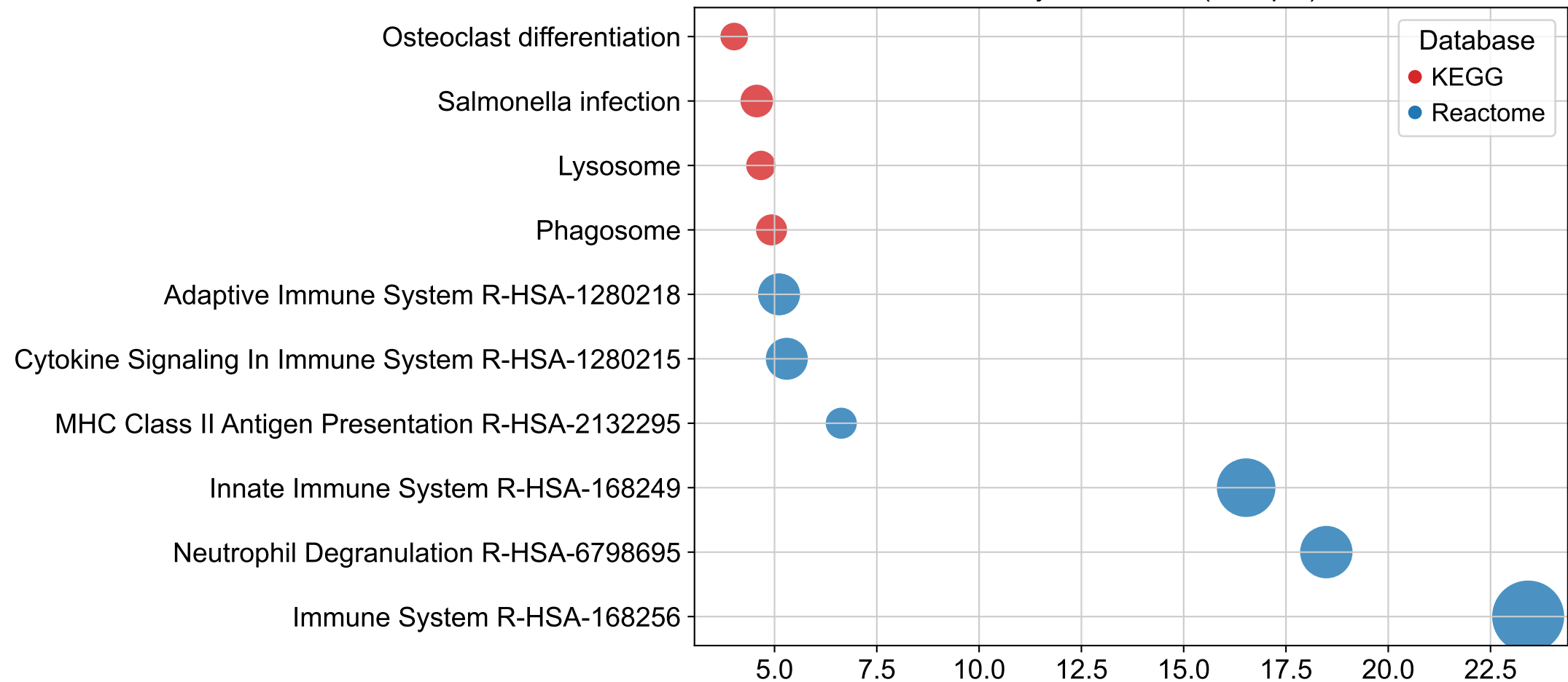
Pathway Enrichment (Group 3)
