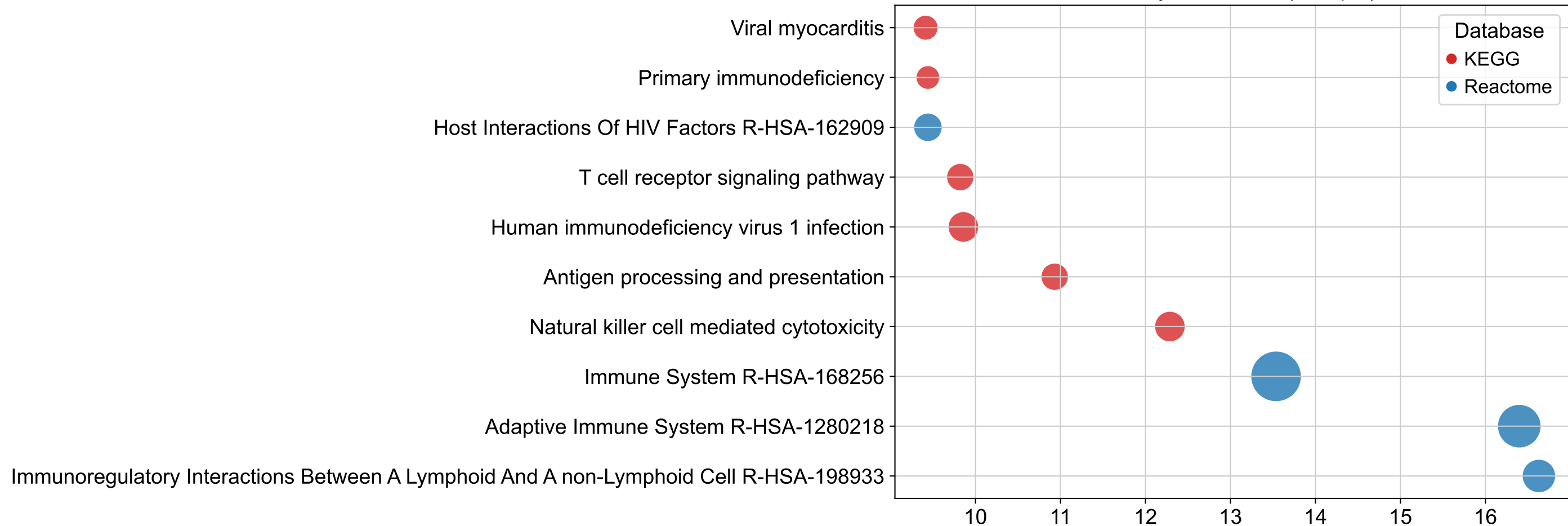
Pathway Enrichment (Group 0)
