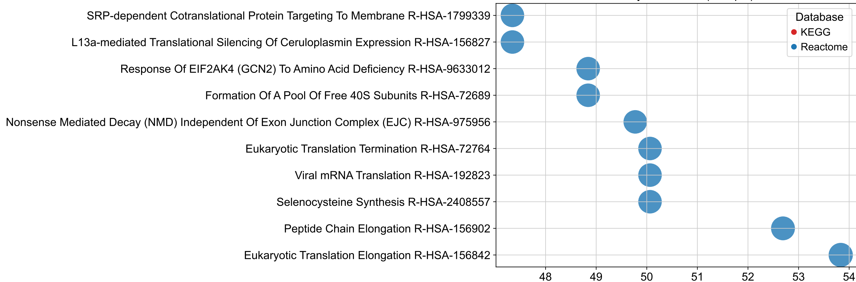
Pathway Enrichment (Group 1)
