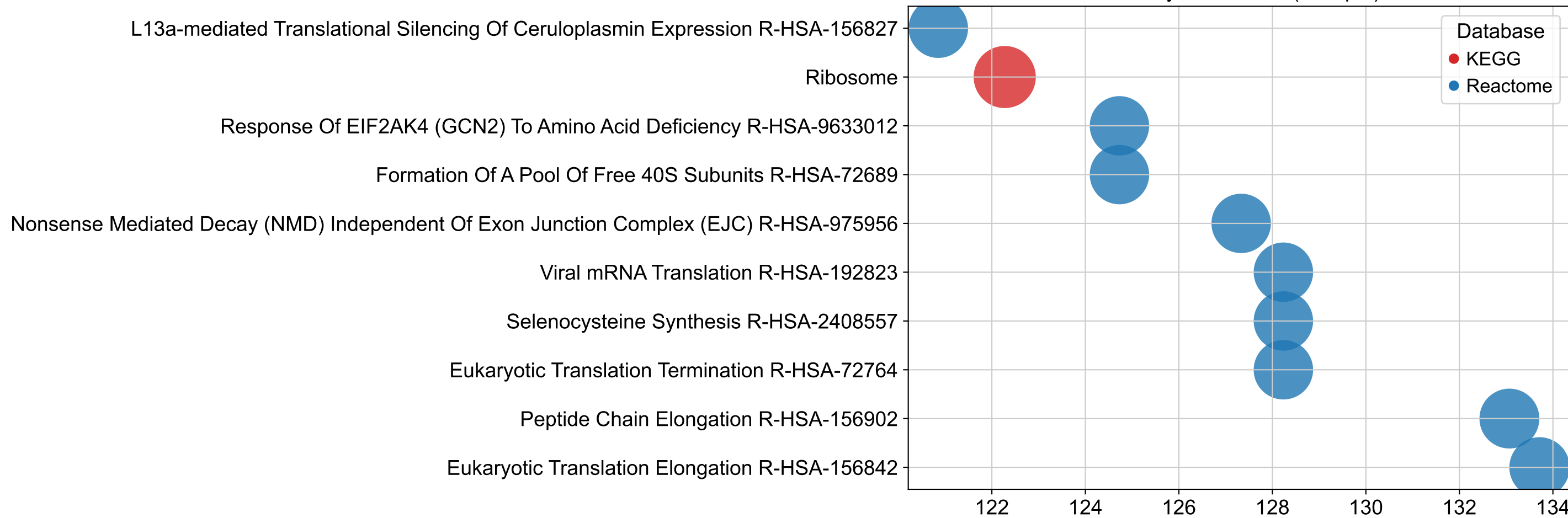
Pathway Enrichment (Group 2)
