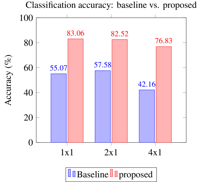
Figure 21: Classification accuracy comparison showing stabilized performance through multi-modal fusion.
