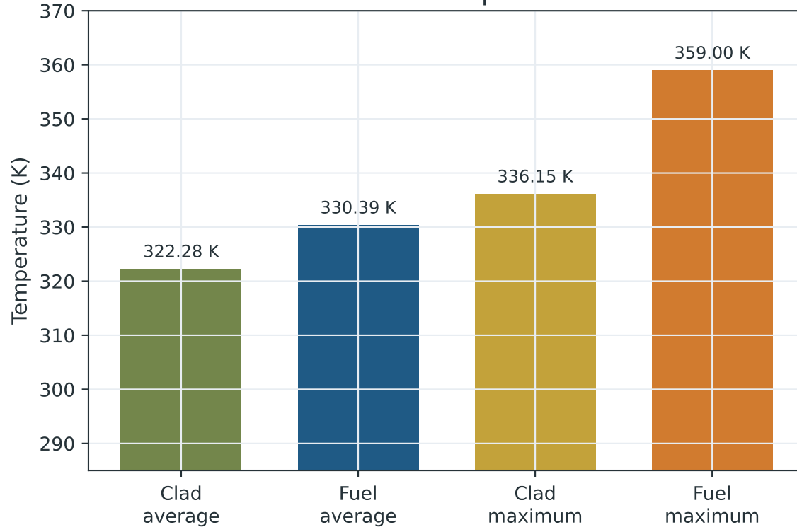
Final solid temperatures
