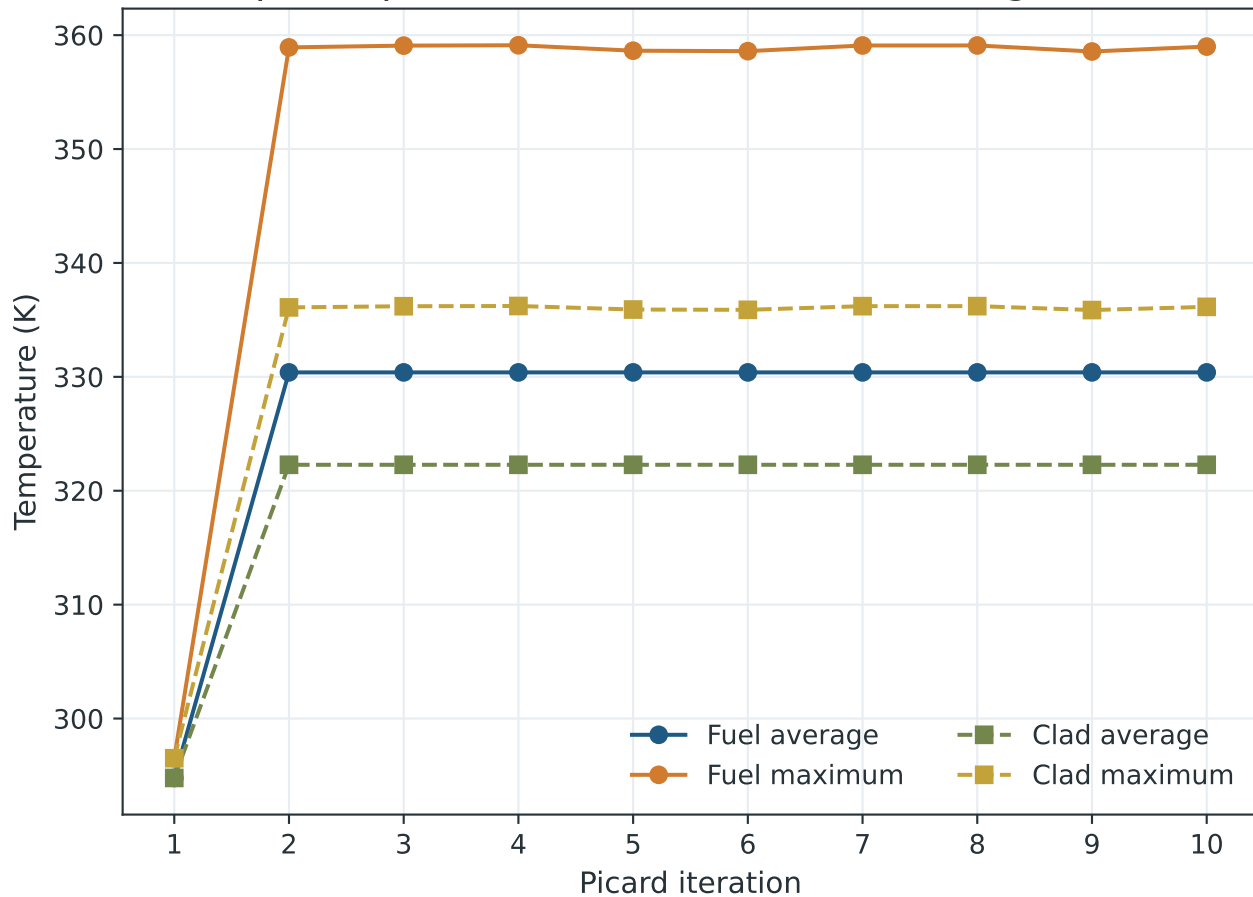
pcM OpenMC-MOOSE thermal convergence
