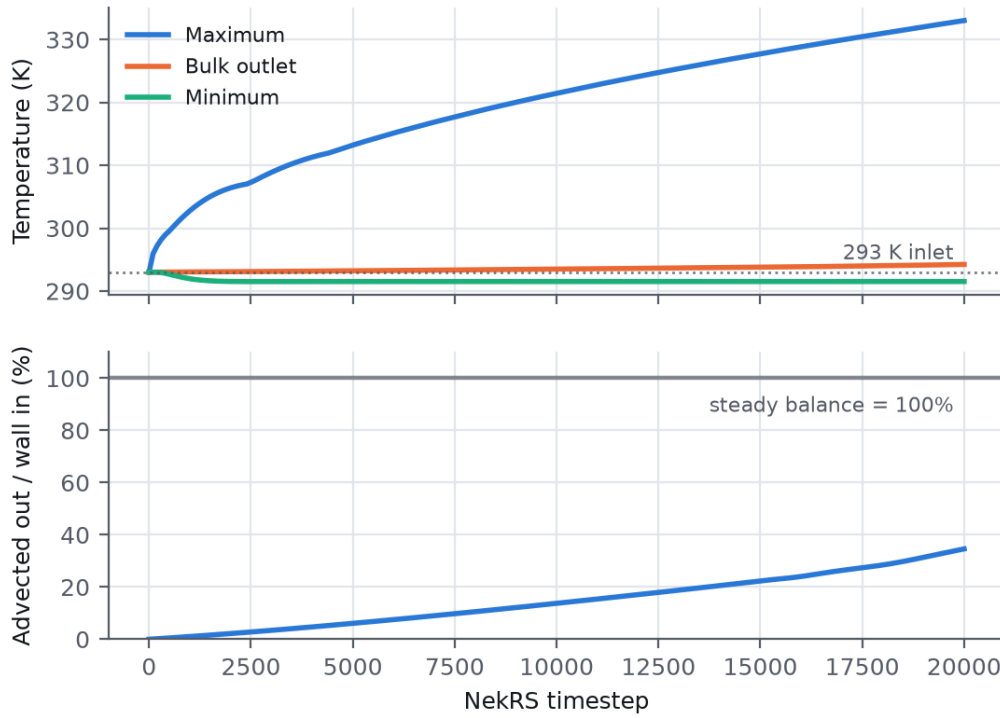
Figure 7. Cardinal NekRS evolution. Upper: coolant temperatures, all still rising at the final step, with the minimum below the 293 K inlet throughout. Lower: energy closure reaches only 34.6% of the steady balance.
