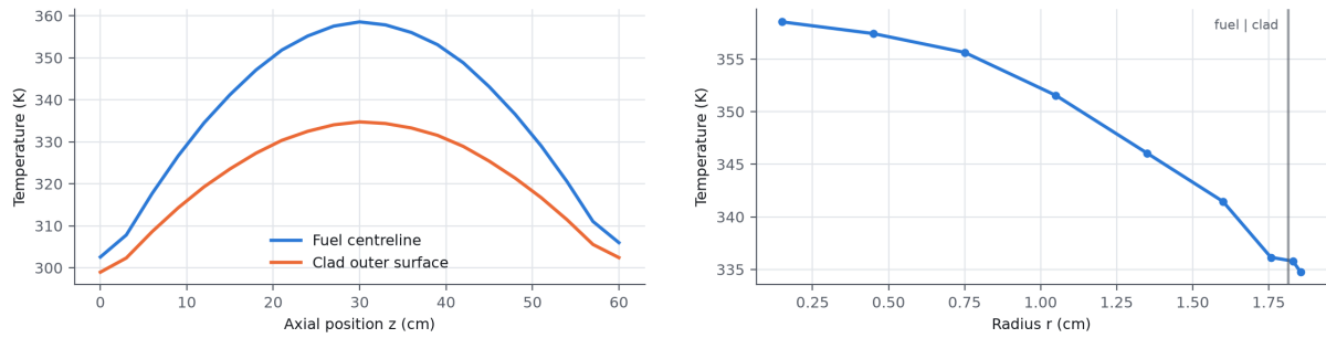
Figure 5. Cardinal coupled temperature solution. Left: axial profile, slightly top-skewed (305.98 K outlet against 302.56 K inlet) because the coolant heats as it rises. Right: radial profile at mid-plane; temperature is continuous across the fuel–clad interface at 1.815 cm, confirming the stitched contact.
