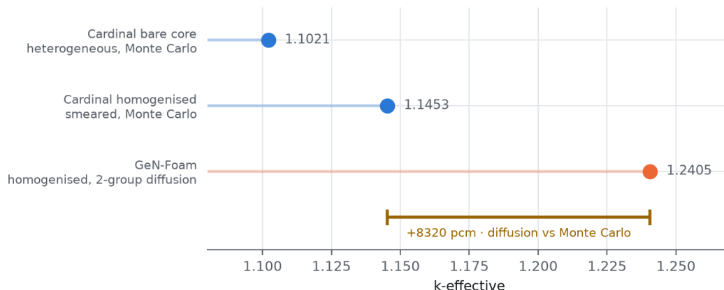
Figure 9. Decomposition of the k_{\text{eff}} difference into a homogenisation step (Monte Carlo on both sides) and a solution-method step (same homogenised bare box).
