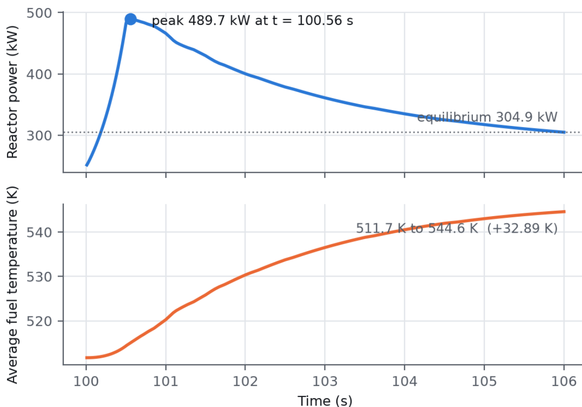
Figure 3. GeN-Foam transient response. Power peaks at 489.7 kW and settles to a Doppler-limited equilibrium of 304.9 kW; average fuel temperature rises 32.89 K.
