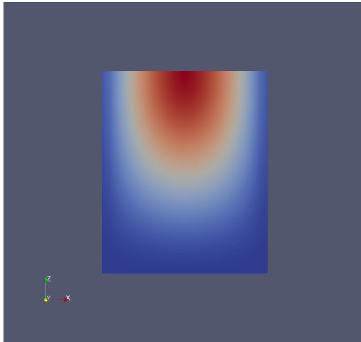
Figure 2. GeN-Foam steady-state temperature field. The maximum lies in the upper portion of the core, consistent with coolant heating as it rises through the channel.
