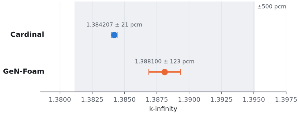
Figure 8. k_\infty comparison. Bars are \pm 1\sigma counting statistics; the shaded band is the 500 pcm acceptance criterion centred on GeN-Foam.
