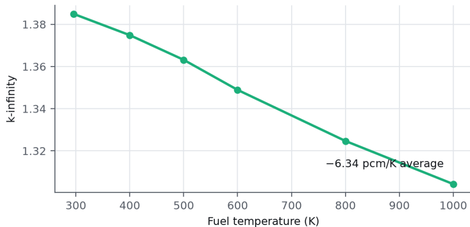
Figure 4. Cardinal fuel temperature coefficient. k_{\infty} falls from 1.384926 at 296 K to 1.304249 at 1000 K.
