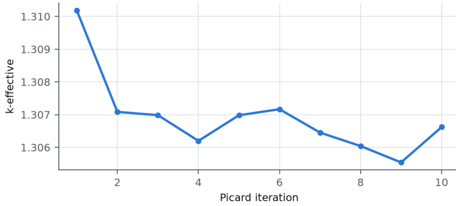
Figure 6. Cardinal Picard convergence. k_{\text{eff}} settles within Monte Carlo noise after the first temperature feedback; average fuel temperature is stable to 10^{-8} K.
