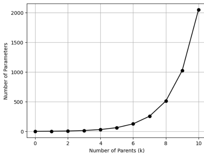
Figure 3.1: A graph that illustrates the exponential growth of CPT parameters
