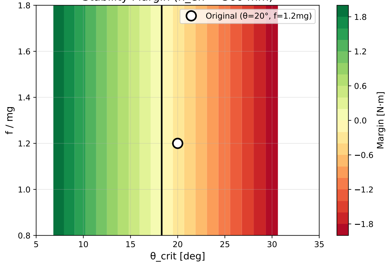
Stability Margin ( h_{\text{eff}} = 360 \text{ mm} )
