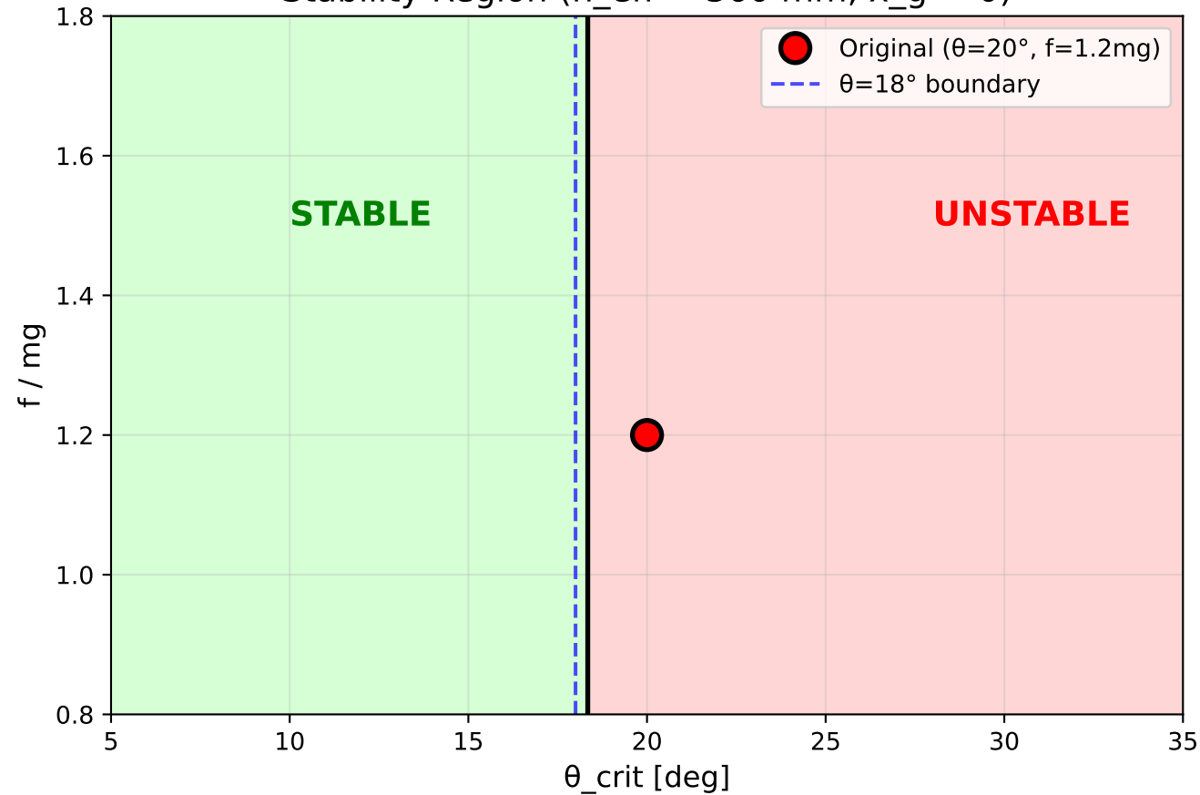
Stability Region ( h_{\text{eff}} = 360 \text{ mm} , x_g = 0 )
