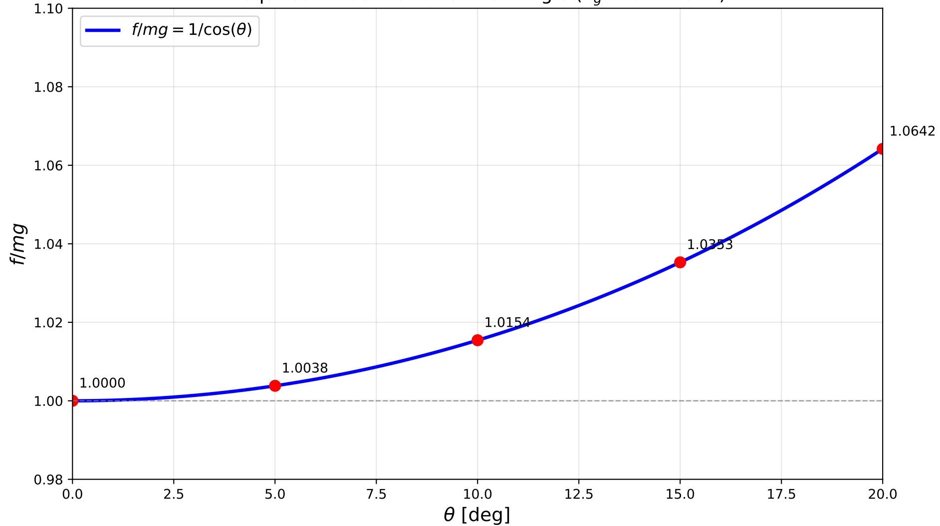
Required Thrust Ratio vs Pitch Angle ( x_g = 0.1275 m)
