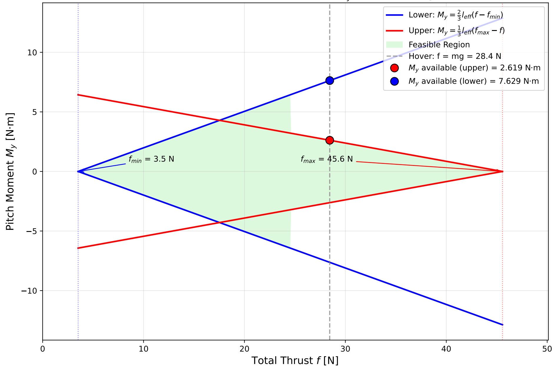
Hexarotor Actuator Constraints: f vs M_y (Diamond Region)
