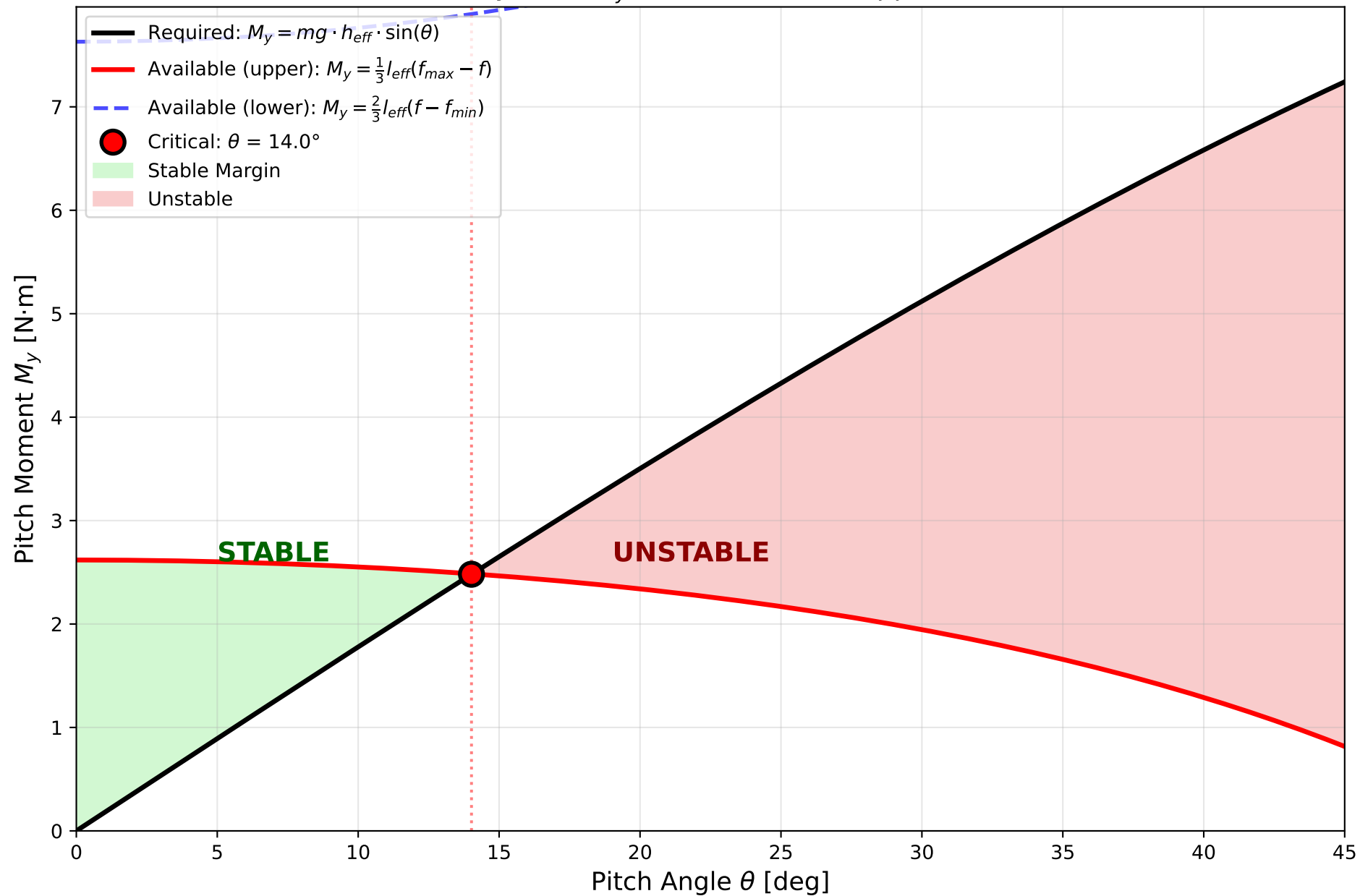
Pitch Stability: \theta vs M_y ( h_{eff} = 360 mm, upper constraint)
