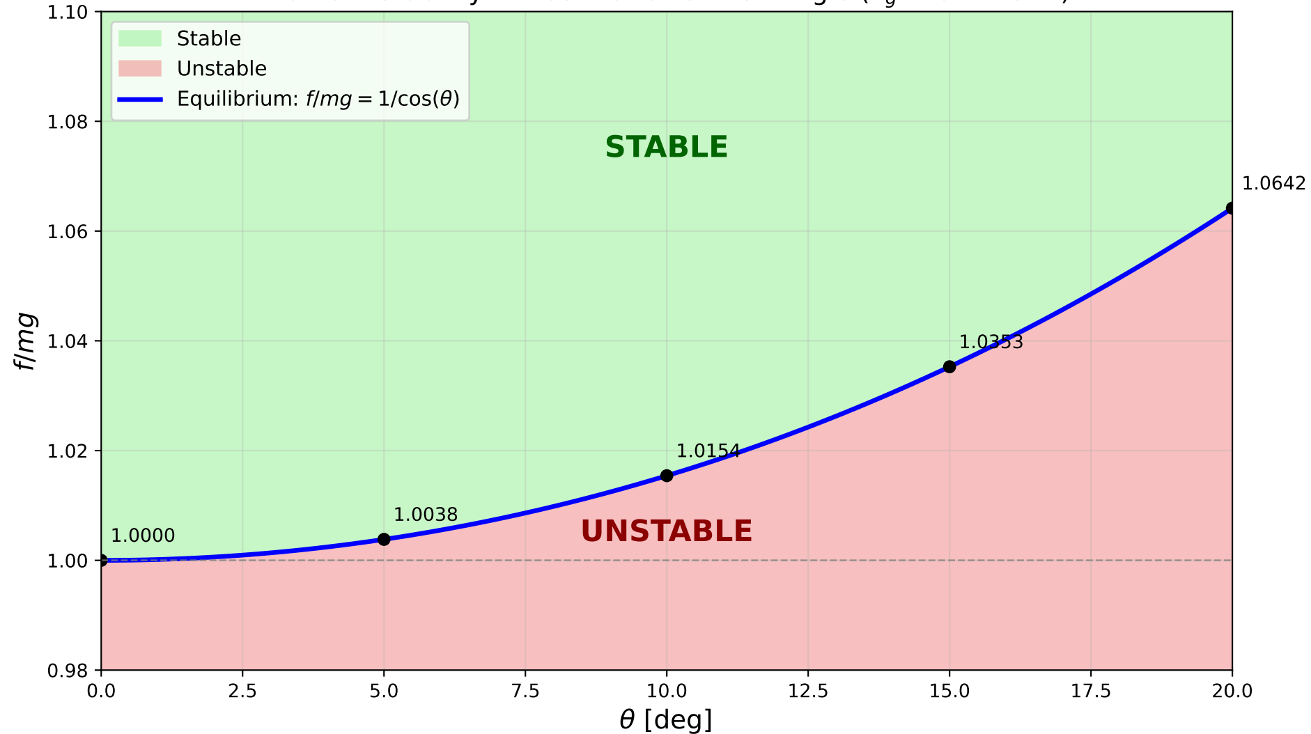
Moment Stability: Thrust Ratio vs Pitch Angle ( x_g = 0.1275 m)
