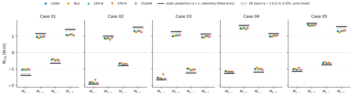
Figure 4: Identified directional critical moments (five estimators, colored markers) against the static-threshold prediction with truth offsets and odometry-fitted arms at \gamma = 1 (black tick); the gray band is the prediction under the ground-effect bracket with the arms held fixed. The markers sit consistently on the smaller-magnitude side of the rigid prediction, move toward the band as \gamma grows, and the residual disagreement is shared by all five estimators — contact physics, not detection.
