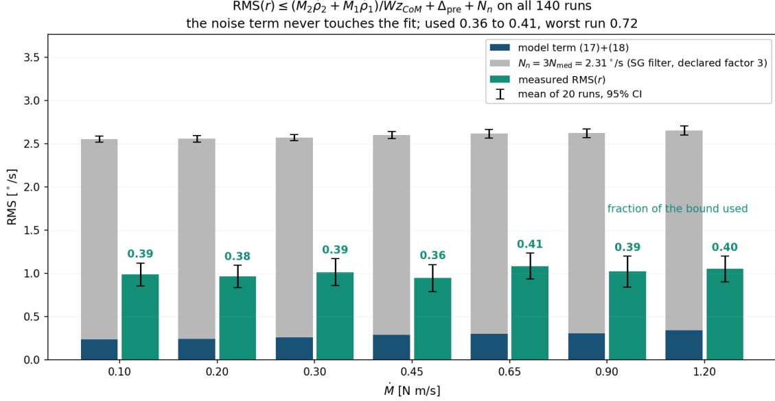
Figure 1: Equation (20) with the adopted noise constant (19b): N_n = 3 N_{med} = 2.31^\circ/\text{s} , three times the campaign median of the Savitzky–Golay high-band anchor ( N_{med} = 0.77^\circ/\text{s} ) — one grey number for every run, no model curve, no minimiser, anywhere in the noise side; the factor is declared up front. Dark blue is the per-run model term, green the measured minimiser residual with 95% intervals; all 140 runs stay inside at used 0.36–0.41, worst run 0.72. For context: the bare minimum total factor for coverage is 2.05; the shape ceiling alone (total 1.96) leaves 2 runs outside; picking a covering quantile would be in-sample calibration; and the campaign maximum with the shape ceiling ( 3.6^\circ/\text{s} ) needs no declared factor at all but costs mean used 0.26. The two halves of the factor do different jobs and neither can absorb the other’s: 1.96 extends a high-band level to the full band under the worst spectral shape (within-run), while 1.5 covers the run-to-run spread of the level itself (max/median = 2.35, between-run) — which is why no shape factor, however large, could replace the level half.
