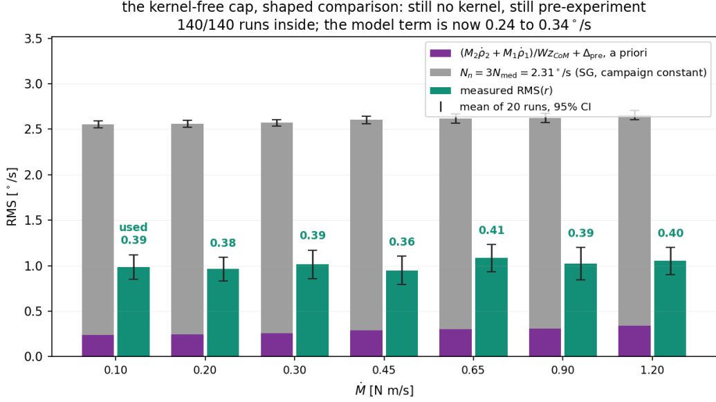
Figure 3: Equation (20) against the campaign: means over the twenty runs at each rate, 95% t intervals. Purple is the model term of (17)+(18), grey the noise constant N_n of (19b), green the measured residual. All 140 runs are inside; the used fraction is 0.36–0.41 and the cap is flat, like the residual.
