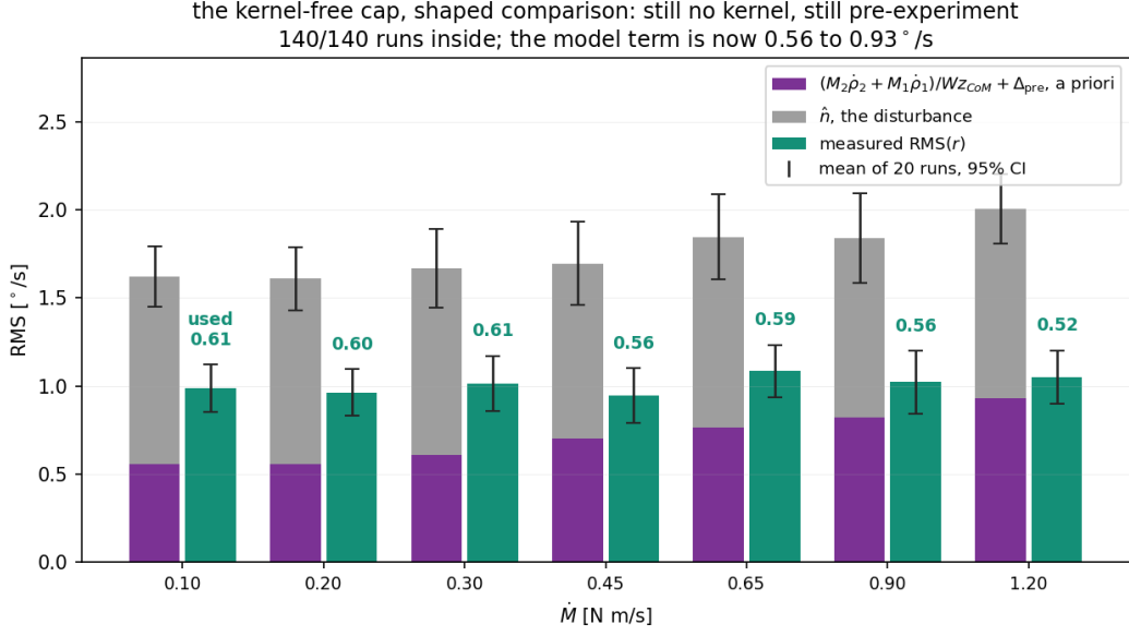
Figure 3: The shaped kernel-free cap, (T.13) + (T.14) + \hat{n} , against the campaign; means over twenty runs per rate with 95% t intervals. The model term is 0.56–0.93°/s — eight times below the constant-forcing version (T.12) and at the level of the projected \Phi — with no kernel computed and every constant available before the experiment. All 140 runs are inside at a used fraction of 0.52–0.61.
