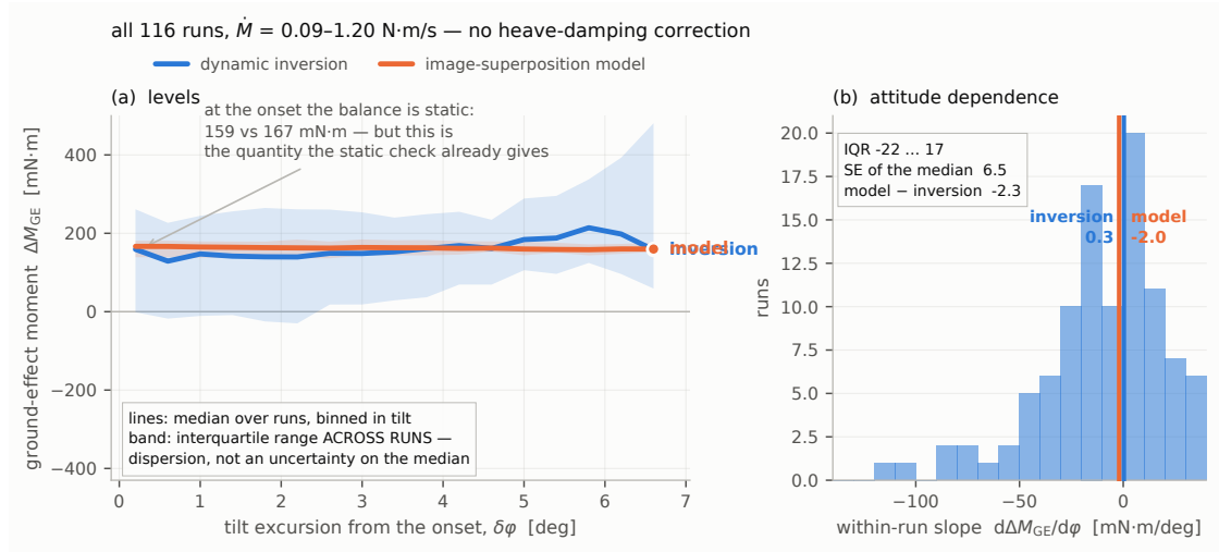
Figure 6: The ground-effect moment from the parameter-free model against the dynamic inversion J_P\dot{\omega} - m - f l_p + W a \cos \varphi - W z_{CoM} \sin \varphi , both plotted against the tilt excursion measured from the onset (median and interquartile band over 116 runs, CAD constants). The levels agree at \delta\varphi = 0 because the balance there is static, so J_P and z_{CoM} drop out and the inversion reduces to the check of Fig. 5. Past about 1^\circ the inversion falls away, reaching -90\text{ mN·m} by 6.5^\circ while the model stays near +155 . The sign of that drift is expected: tipping about one foot lifts the opposite rotors clear of the ground, and those carry the long moment arms, so the net ground-effect moment must fall with tilt — the model’s own slope is negative too, -2.7 to -0.1\text{ mN·m/deg} . What the inversion cannot be measuring is the magnitude, sixteen times larger, nor the crossing into a net restoring moment, which would need the near-pivot rotors to outweigh the far ones. The drift is the residual of the W z_{CoM} \sin \varphi cancellation, and the model’s slope sits inside its linewidth. The attitude dependence of the ground-effect moment is therefore bounded by the excitation design — the tilt cap — rather than measured.
