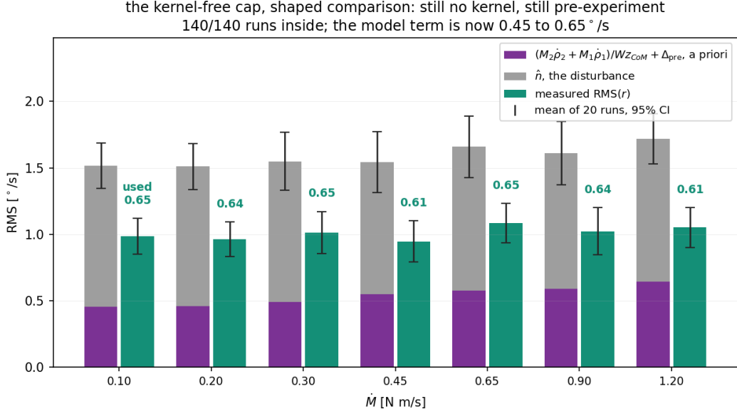
Figure 2: Equation (20) against the campaign: means over the twenty runs at each rate, 95% t intervals. Purple is the model term of (17)+(18), grey the noise estimate (19), green the measured residual. All 140 runs are inside; the used fraction is 0.61–0.65 and the cap is flat, like the residual.
