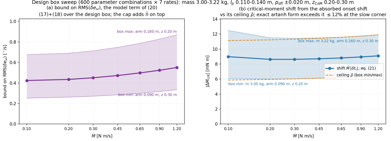
Figure 3: The design-box sweep. (a) the bound on \text{RMS}(\delta e_\omega) , eq. (17)+(18): 0.25\text{--}0.87^\circ/\text{s} over box and rates, median 0.42\text{--}0.55 . The band is set by the ratio \text{arm}/z_{CoM} — worst at arm 0.160 m with z_{CoM} = 0.20 m, best at arm 0.090 m with 0.30 m. (b) the critical-moment shift M|\delta t_c| of (21): 6.0\text{--}12.5 mNm, tracking its ceiling \bar{\rho} and exceeding it by at most 12\% at the slow-ramp corner — the \text{artanh}(u)/u factor of the exact shift — while flat in \dot{M} by the cancellation. Its worst corner has the opposite z direction — m = 3.22 kg, arm 0.160 m, z_{CoM} = 0.30 m — because \bar{\rho} grows with the window that a higher CoM lengthens, while the residual bound worsens with \text{arm}/z_{CoM} .
