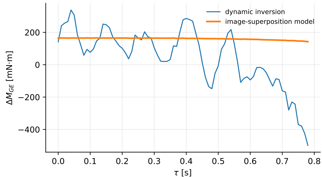
case_02/Mx/pos_Mx_01 ( z_{CoM} = 0.261 m, J_P = 0.220 kg m 2 )
