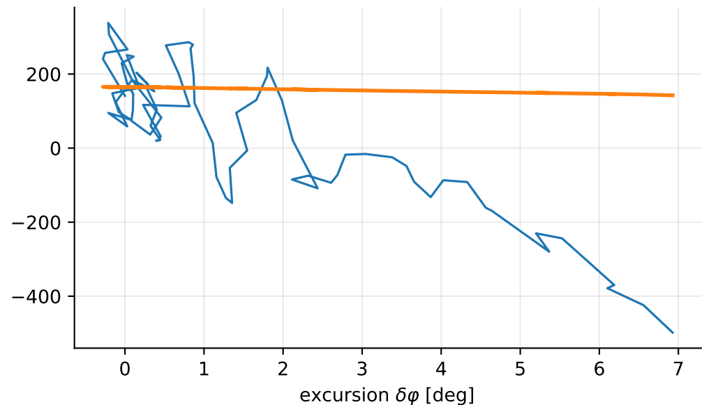
case_02/Mx/pos_Mx_01 ( z_{CoM} = 0.261 m, J_P = 0.220 kg m 2 )
