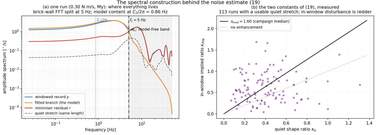
Figure 1: The spectral construction of (19). (a) One run’s amplitude spectra: the fitted branch (the model) collapses above a few hertz, so past the 5 Hz split the residual coincides with the record — pure disturbance, the anchor n_{hi} ; a quiet stretch of the same length gives the shape ratio \kappa_q . Spectra are Hann-tapered and zero-padded for display only — the numbers in (19) use the raw bins of the residual, where the branch has been subtracted and edge leakage cancels. (b) The in-window implied ratio against the quiet ratio over the 113 runs with a usable quiet stretch; the in-window disturbance is redder, by the campaign-median factor s_{med} = 1.60 .
