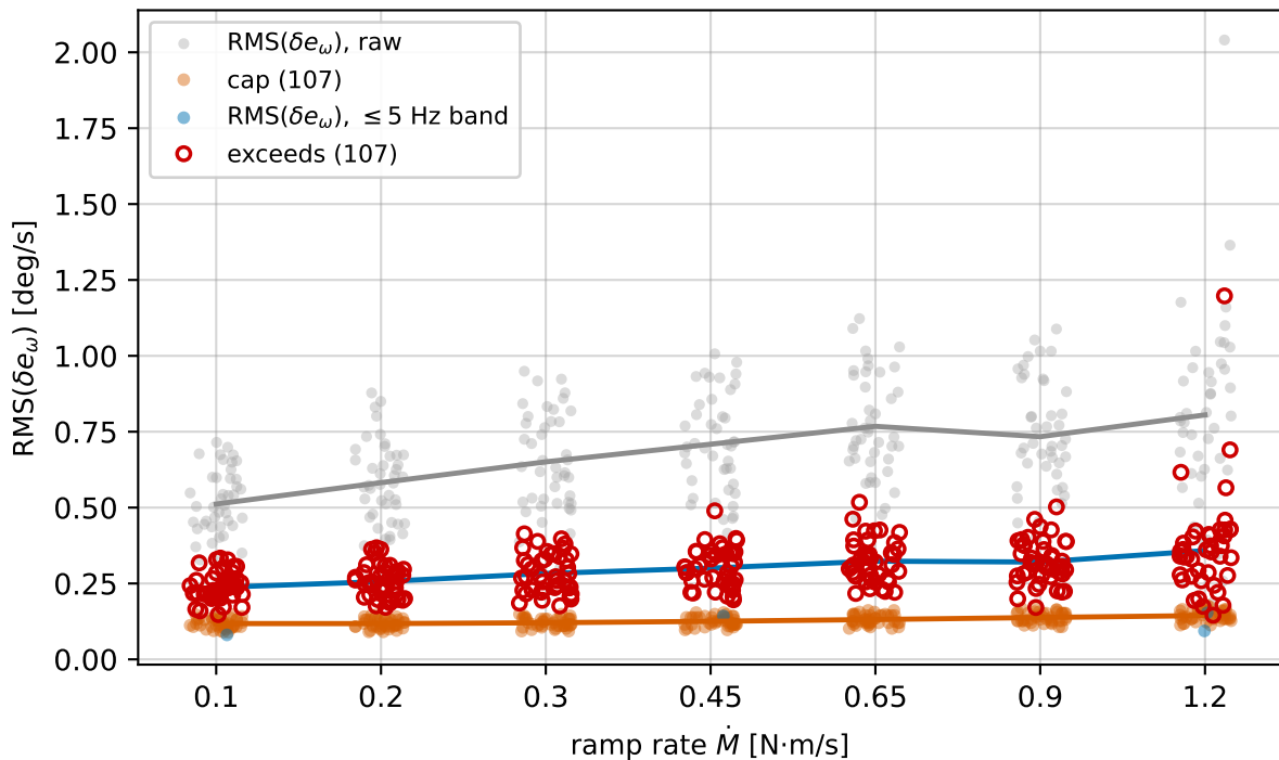
simulation, design tilt cap 5°: 4/301 inside (low band)
