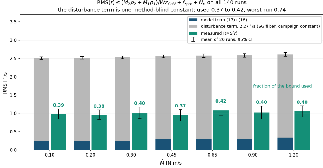
Figure 1: Equation (20) with the method-blind noise constant, the adopted form: 1.5 \times the median Savitzky–Golay anchor ( N_{med} = 0.77^\circ/\text{s} ), times \sqrt{1 + \kappa_{sup}^2} — one grey number, 2.27^\circ/\text{s} , for every run, no model curve anywhere in the noise side; the safety factor is declared up front. Dark blue is the per-run model term, green the measured minimiser residual with 95% intervals; all 140 runs stay inside at used 0.37–0.42, worst run 0.74. For context: the bare minimum factor for coverage is 1.05; the median alone ( k = 1 ) leaves 2 runs outside (worst 1.04 \times ); picking a covering quantile (p75) would be in-sample calibration; and the campaign maximum — equivalent to k = 2.35 — needs no declared factor at all but costs mean used 0.26.
