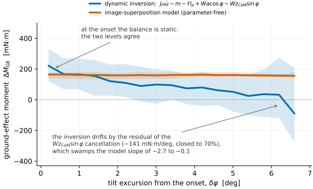
Figure 6: The ground-effect moment from the parameter-free model against the dynamic inversion J_P \dot{\omega} - m - f l_p + W a \cos \varphi - W z_{CoM} \sin \varphi , both plotted against the tilt excursion measured from the onset (median and interquartile band over 116 runs, CAD constants). The levels agree at \delta\varphi = 0 because the balance there is static, so J_P and z_{CoM} drop out and the inversion reduces to the check of Fig. 5. Past about 1^\circ the inversion walks away, reaching -90 mN m by 6.5^\circ while the model stays near +155 : that drift is the residual of the W z_{CoM} \sin \varphi cancellation, not a measured attitude dependence. The model's own slope, -2.7 to -0.1 mN m/deg, is inside the linewidth. The attitude dependence of the ground-effect moment is therefore bounded by the excitation design — the tilt cap — rather than measured.
