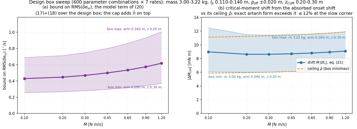
Figure 3: The design-box sweep. (a) the bound on RMS(\delta e_\omega) , eq. (17)+(18): 0.26\text{--}1.00^\circ/s over box and rates, median 0.43\text{--}0.62 . The band is set by the ratio arm/z_{CoM} — worst at arm 0.160 m with z_{CoM} = 0.20 m, best at arm 0.090 m with 0.30 m. (b) the critical-moment shift M|\delta t_c| of (21): 6.0\text{--}12.5 mN m, tracking its ceiling \bar{\rho} and exceeding it by at most 12\% at the slow-ramp corner — the \text{artanh}(u)/u factor of the exact shift — while flat in \dot{M} by the cancellation. Its worst corner has the opposite z direction — m = 3.22 kg, arm 0.160 m, z_{CoM} = 0.30 m — because \bar{\rho} grows with the window that a higher CoM lengthens, while the residual bound worsens with arm/z_{CoM} .
