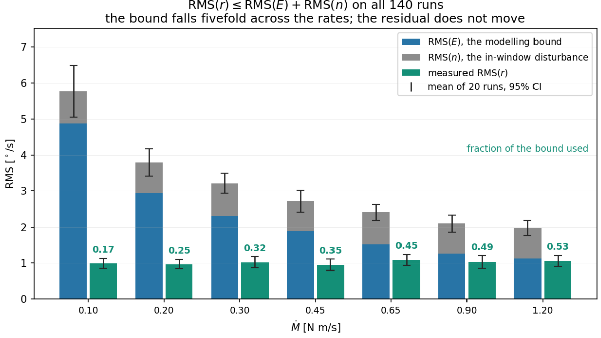
Figure 2: (VIII.3) on the campaign: the full residual against the cap \text{RMS}(E) + \text{RMS}(n) at each ramp rate, means over the twenty runs with 95% t intervals. What moves is the cap, not the residual — it falls from 5.77 to 1.98^\circ/\text{s} while the measured residual stays between 0.95 and 1.08 , its intervals overlapping throughout — so the fraction of the bound used climbs from 0.17 to 0.53 because the guarantee tightens, not because the fit deteriorates.
