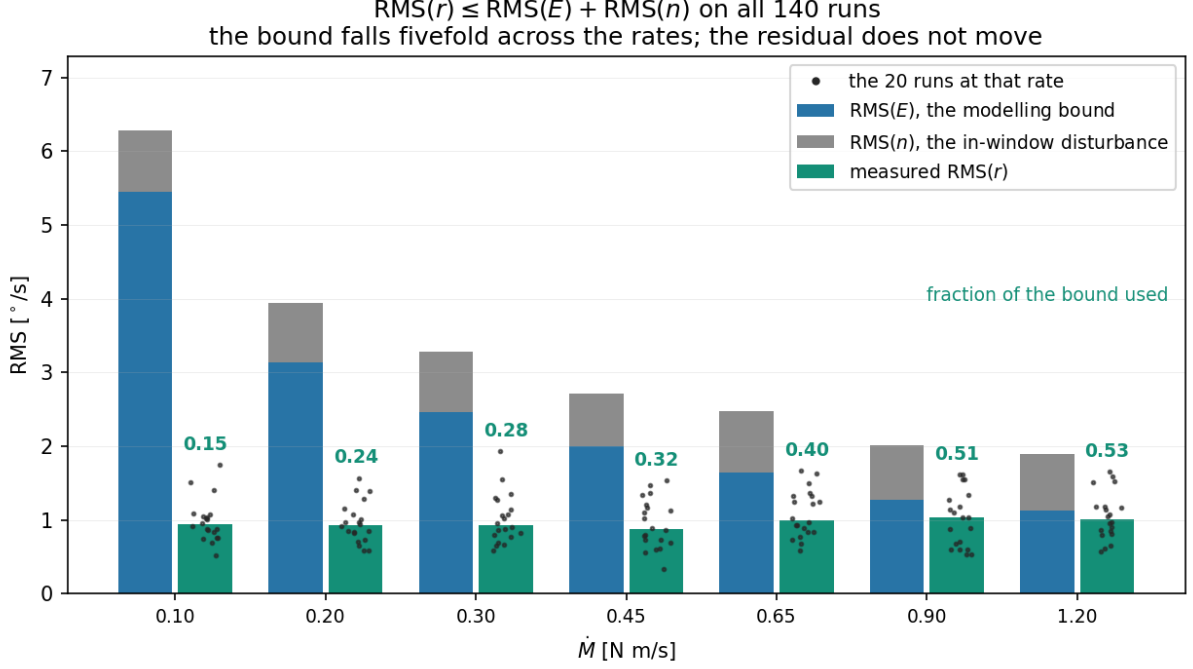
Figure 2: (VIII.3) on the campaign: the full residual against the cap \text{RMS}(E) + \text{RMS}(n) , at each ramp rate, with the twenty runs of that rate as points. What moves is the cap, not the residual — \text{RMS}(E) falls from 5.46 to 1.13^\circ/\text{s} while the measured residual stays between 0.88 and 1.03 — so the fraction of the bound used climbs from 0.15 to 0.53 because the guarantee tightens, not because the fit deteriorates.
