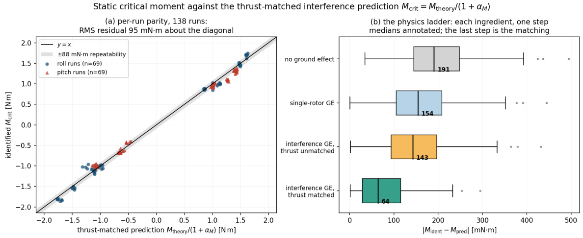
Figure 6: The matched-thrust comparison, per run. (a) Parity of the identified M_{\text{crit}} against M_{\text{theory}}/(1 + \alpha_M) over the 138 runs with a valid pivot fit: both tip directions sit on the diagonal within the \pm 88 mN m static repeatability band (RMS 95 mN m). (b) Per-run |residual| as one physics ingredient is added per step: no ground effect (191 mN m median), single-rotor ground effect (154), the interference model with the thrust channel dropped from the reference (143), and the full matched-thrust interference prediction (64). The largest single step is the thrust matching itself. (Per-run medians; the group-mean medians of Table 13 differ slightly by aggregation.)
