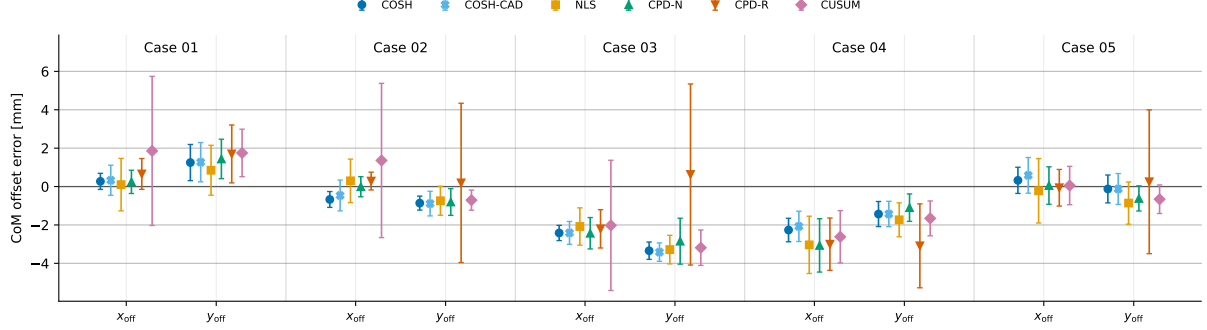
Figure 4: The same data folded about the truth: CoM offset error (estimate – truth) with 95% confidence intervals, grouped by component within each case ( x_{\text{off}} from the pitch excitation, y_{\text{off}} from the roll excitation). The residual biases of cases 3 and 4 are common to every estimator — a vehicle–contact asymmetry, not a detection artifact — while the estimator-to-estimator differences stay within about \pm 1 mm.
