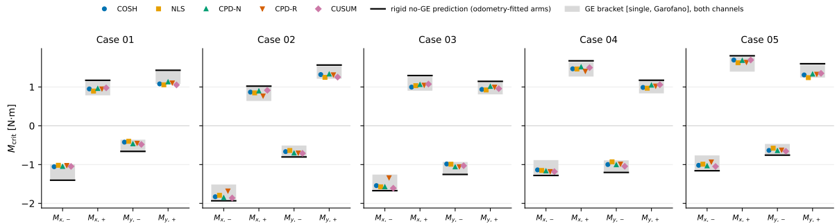
Figure 4: Identified directional critical moments (five estimators, colored markers) against the rigid no-GE static prediction (black tick) and the first-principles ground-effect bracket (gray band spanning the single-rotor and Garofano-adapted predictions, both channels, arms fixed). The identified thresholds fall inside the band in 19 of 20 groups.
