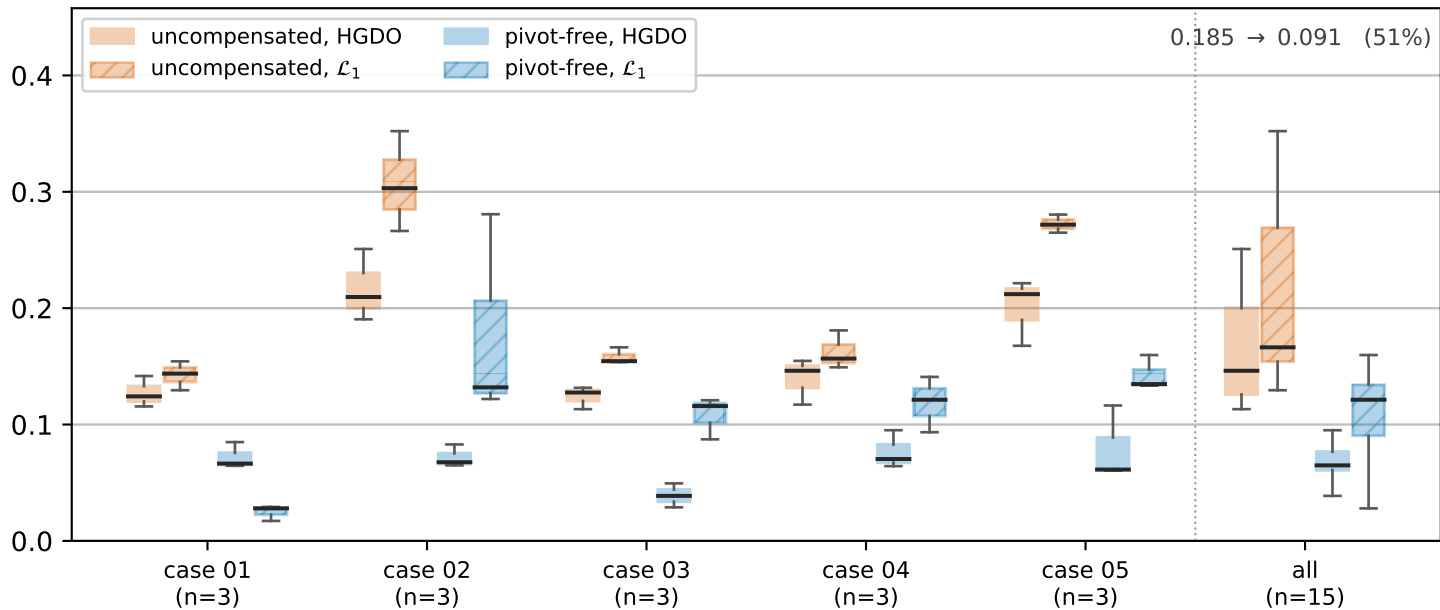
peak horizontal drift [m]
